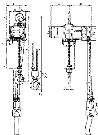
Modell CPA 1-13 / 2-10 / 5-5
